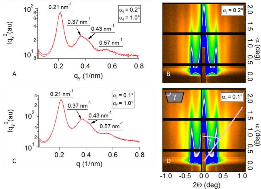
Figure 2.14 GISAXS measurement of films by solvent annealing under PGMEA: (A,B) above the polymer's critical angle, sampling the full film thickness; (C,D) below the polymer's critical angle, sampling the top ~10 nm.
